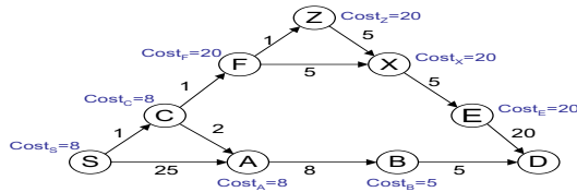
Fig. 1. Cross-layer routing
