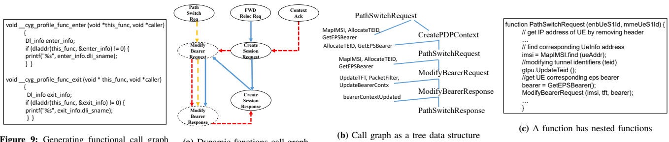
Figure 9: Generating functional call graph through gcc instrument functions
