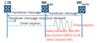
Figure 7: Expiry of timer between two NFs has a domino effect that leads to an event failure
