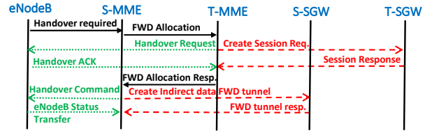
Figure 12: Concurrent execution of messages: S1AP messages (shown as dotted line arrows) and GTP messages (shown as dashed line arrows) are executed in parallel to each other. Sequence execution of messages (S1AP and GTP) are shown as solid line
