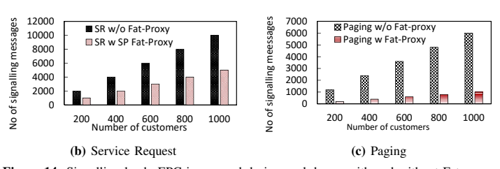
Figure 14: Signalling load vEPC is exposed during peak hours with and without Fat-proxy
